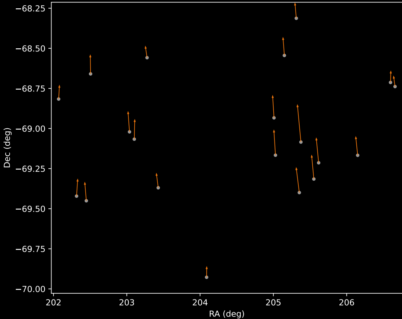
GALAH DR4 Cluster 2 Proper Motion Vectors (n=20)
