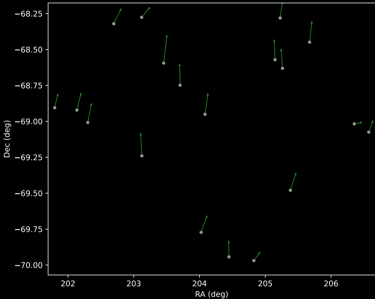
GALAH DR4 Cluster 4 Proper Motion Vectors (n=19)
