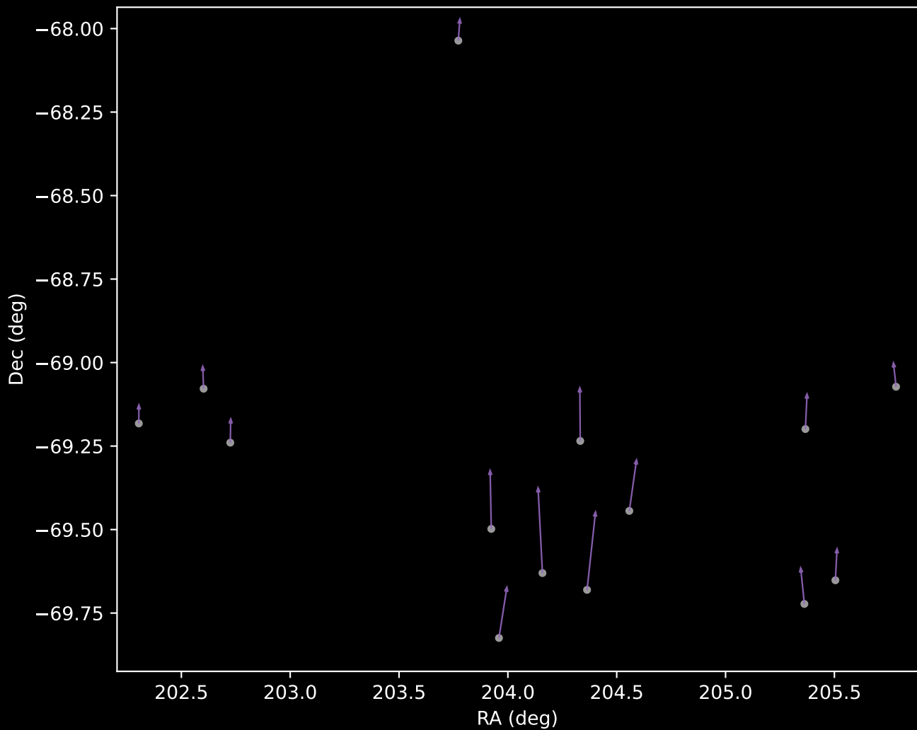
GALAH DR4 Cluster 8 Proper Motion Vectors (n=14)
