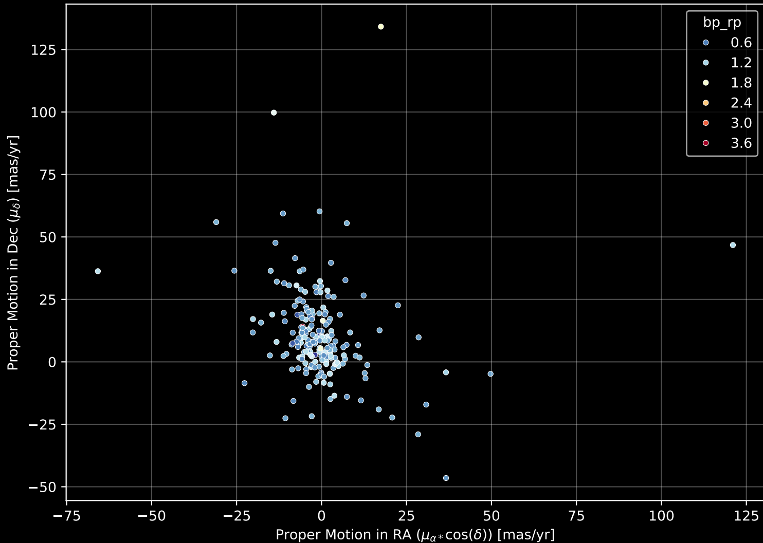
GALAH DR4 Field: [7147] Proper Motion Diagram (n= 215)
