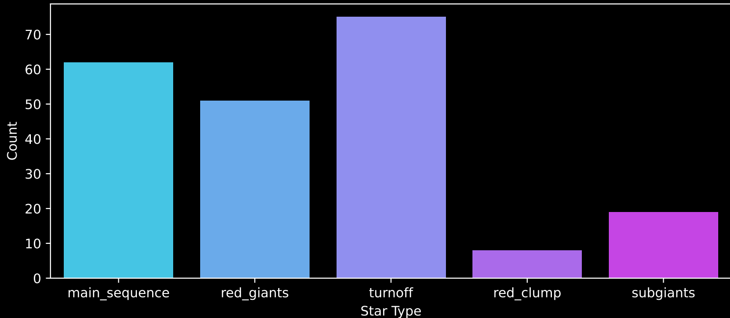
GALAH DR4 Field: [7147] Count plot of Star Type
