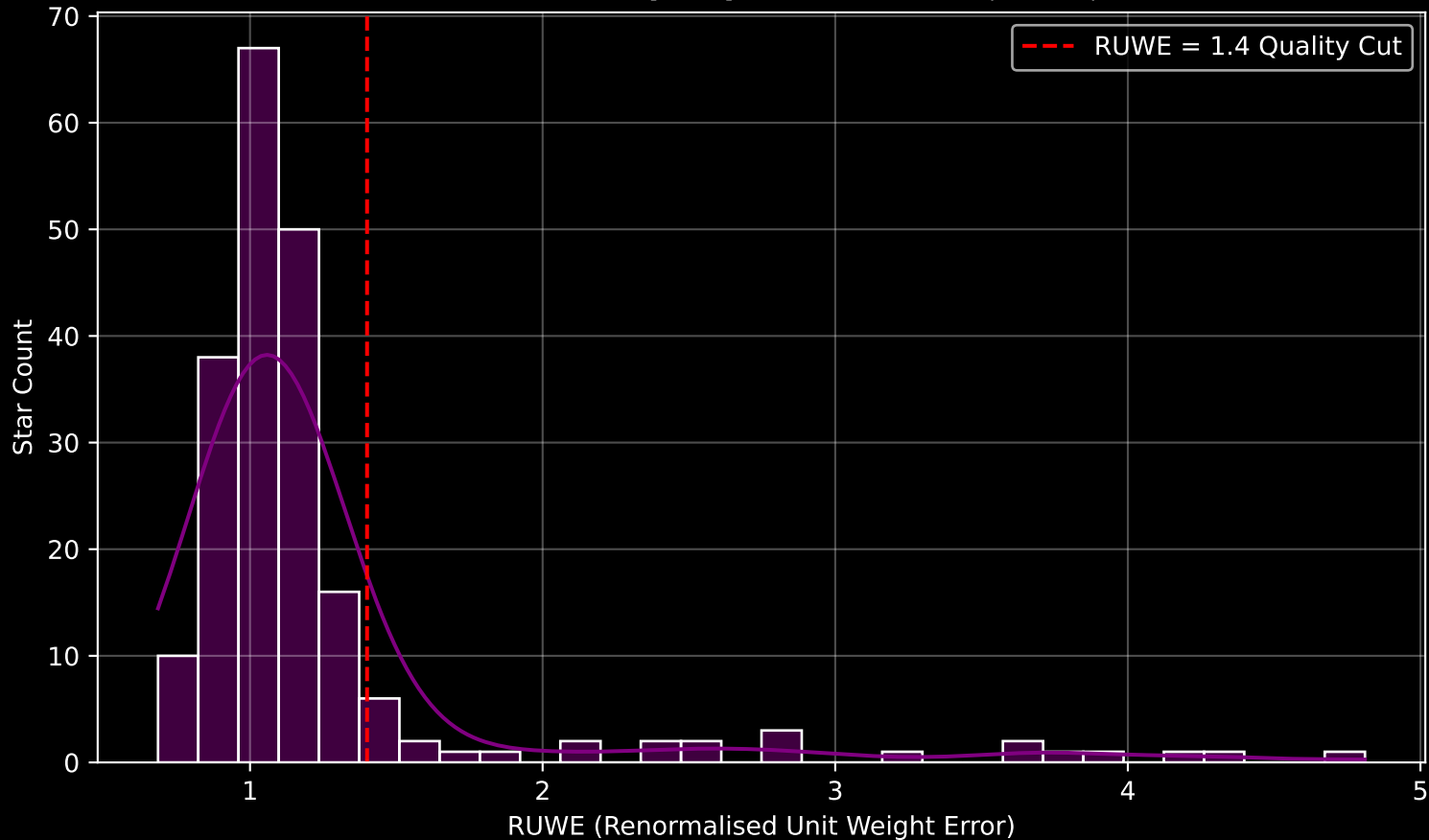
GALAH DR4 Field [7147] RUWE Distribution (n= 208)
